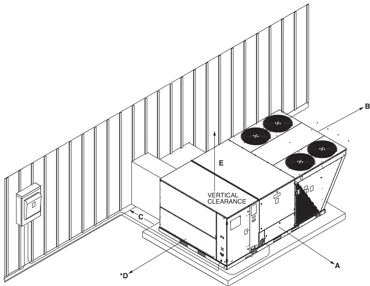
Illustration ST-A1326-49
