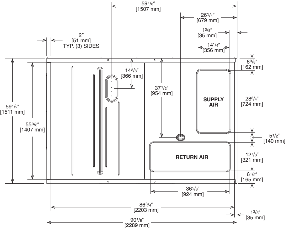
Illustration ST-A1273-01_A-01
