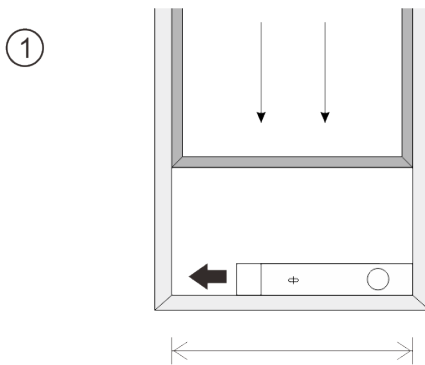
Window width Min: 40cm Max: 120cm Fig.4
