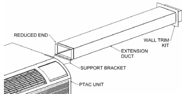
Figure 8 – Extension Duct Attachment
