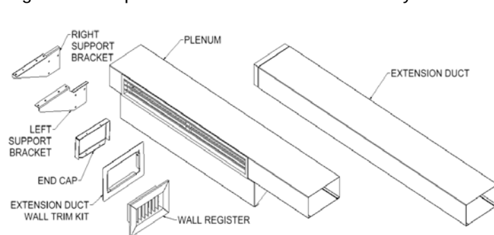
Figure 1- Components for Lateral Duct Accessory Kit
