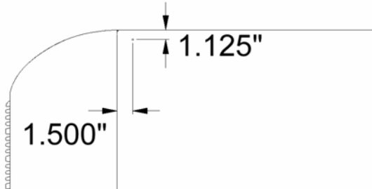
Figure 2 – Side View of Metal Wall Sleeve showing measurements for Top Hole Location.
